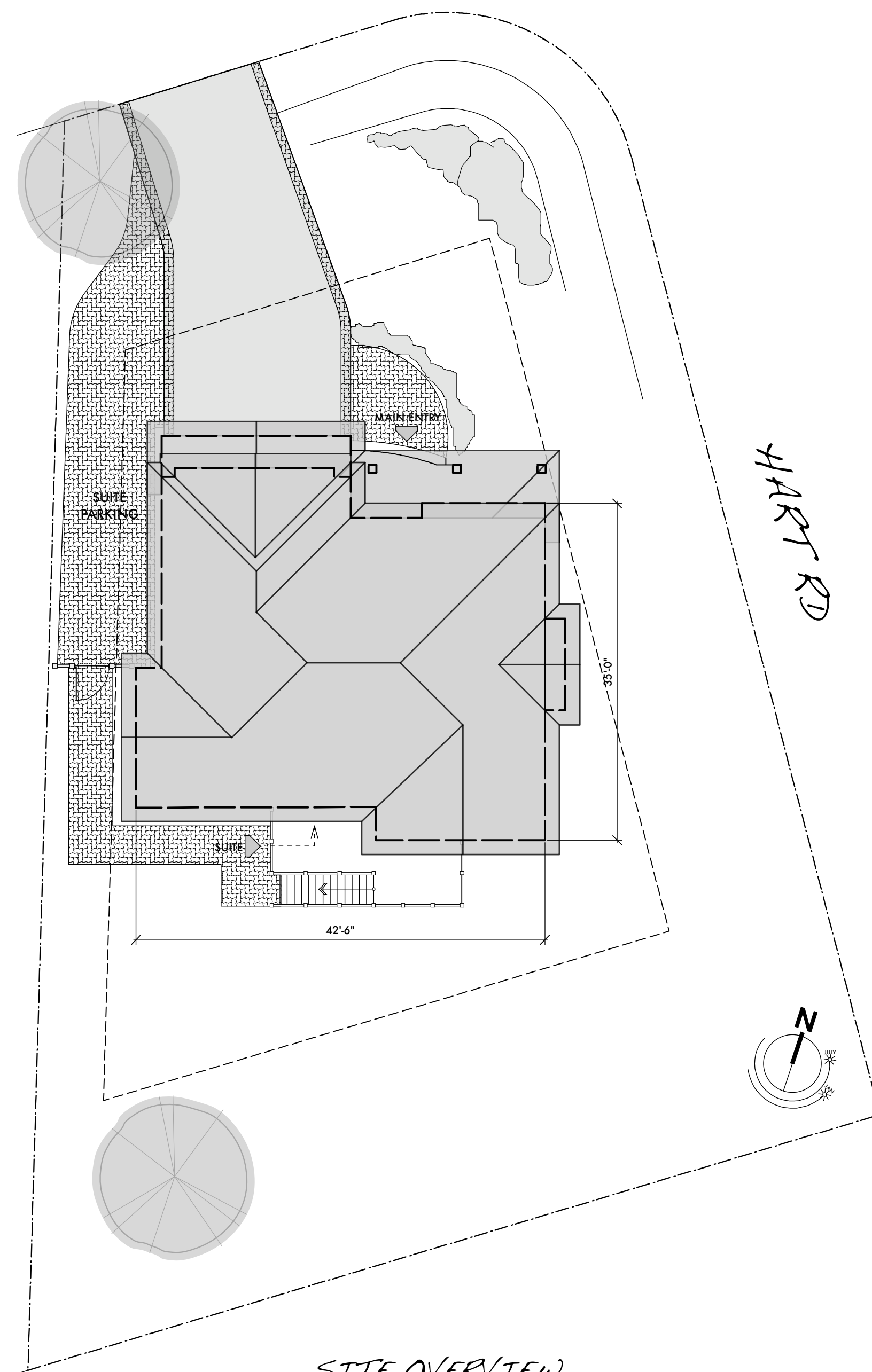
SITE OVERVIEW 3/32"=1'-0"
