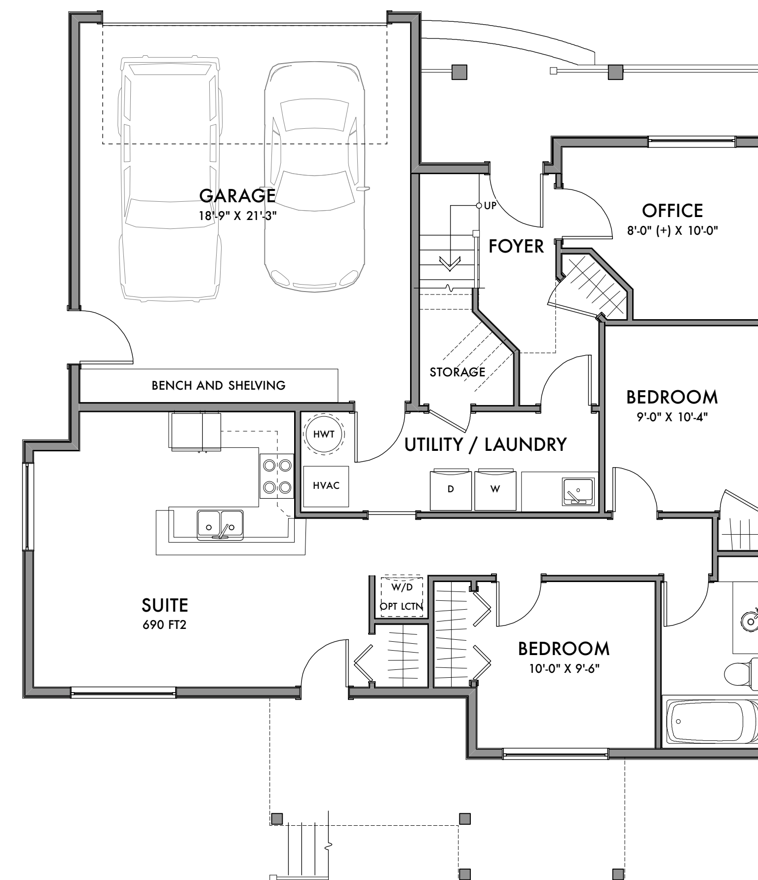
LOWER FLOOR PLAN 3/16"=1'-0"
